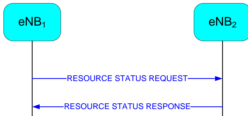
Fig. 2-27: Resource Status communication between eNBs
