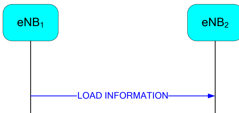
Fig. 2-26: Load information exchange between eNBs
