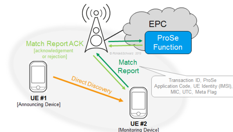
Fig. 2-13: Direct Discovery and Match Report
