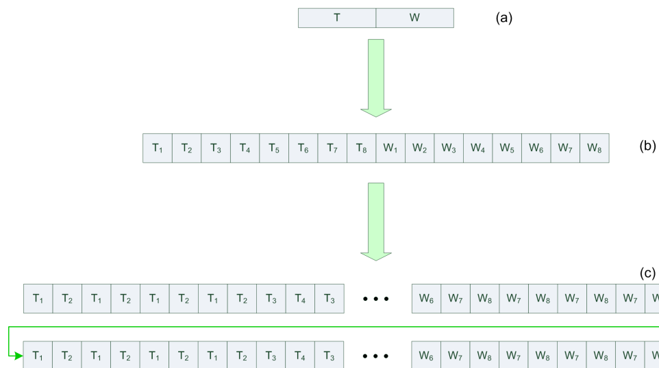
Figure 5-5: Example of an arrangement for NPUSCH transmission with repetitions. For the case of no repetitions, the slot sequence shown in (b) would be transmitted.
