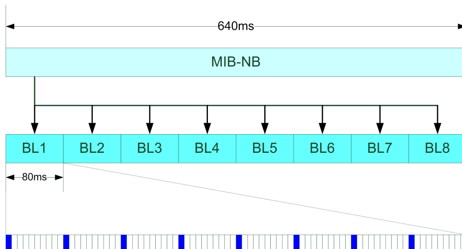
Figure 3-7: NPBCH mapping to the subframes
