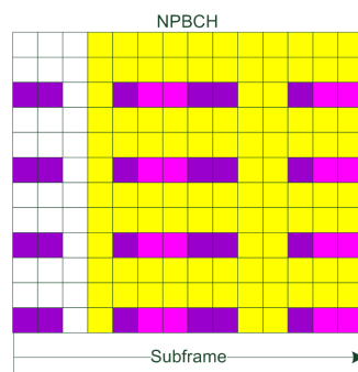
Figure 3-8: Resource element occupation of the NPBCH indicated in yellow. In magenta, the NRS are shown, and in violet, the CRS.
