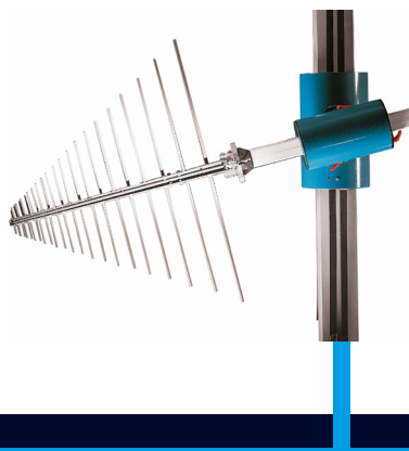
Log-periodic antenna R&S®HL223 200 MHz to 1000 MHz
