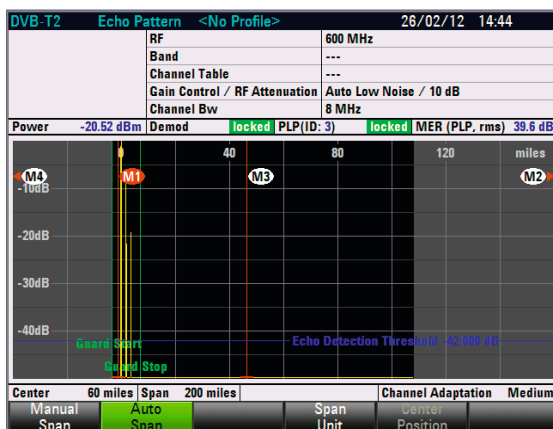
Channel impulse response.
