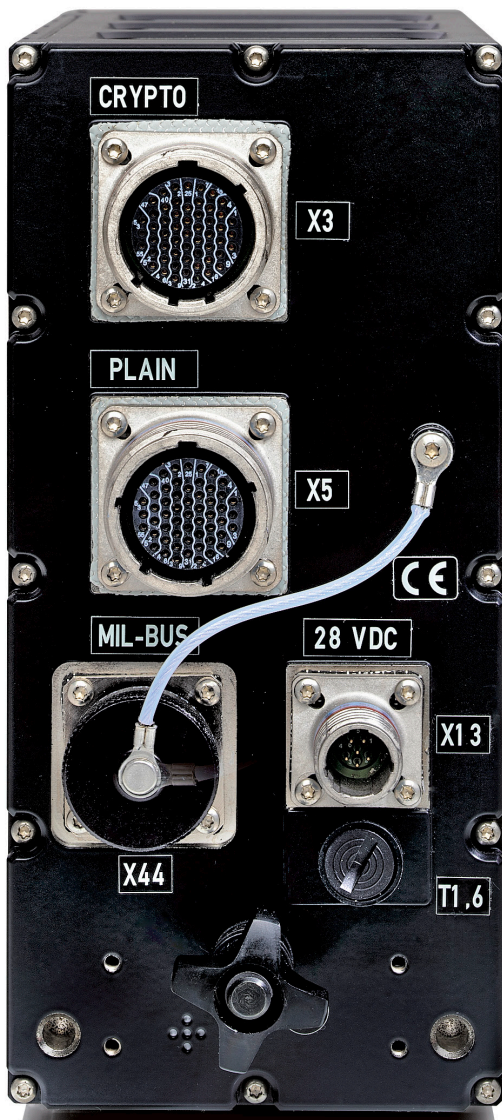
Rear view of the R&S®MMC3000
