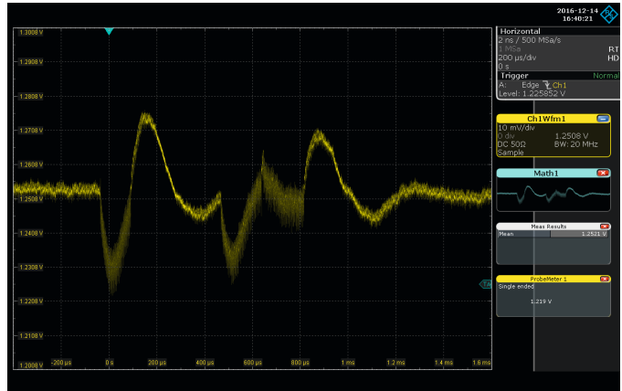
Load response measurement of a DDR4 power supply during initialization phase of the DDR memory.
