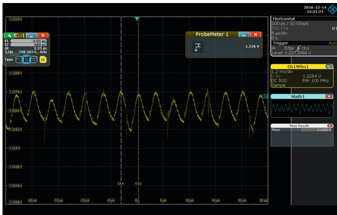
Measuring remaining ripple on a 1.2 V DDR4 power supply and accurately verifying the DC level with the R&S®ProbeMeter, a DC voltmeter integrated into the probe head.
