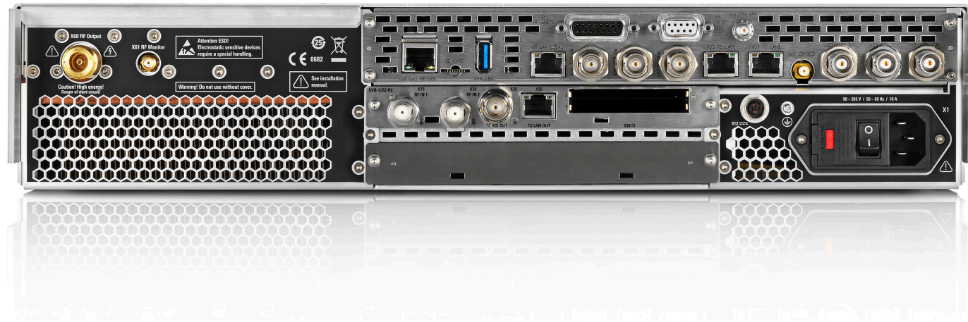
The transmitters of the R&S®TLx9 family have free slots to accommodate hardware options for expanded functionality.
