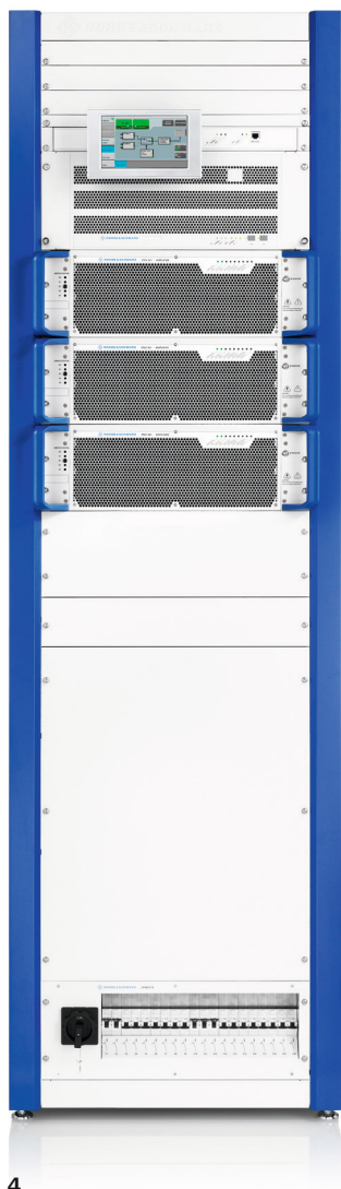
R&S®TMV9 transmitter with three amplifiers and an output power of 2.2 kW (DAB and DTV).
