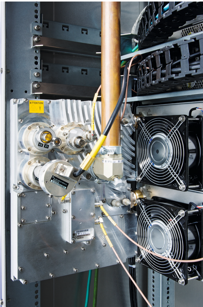
6-in-1 coupler unit for coupling two R&S®PMU901 amplifiers.
