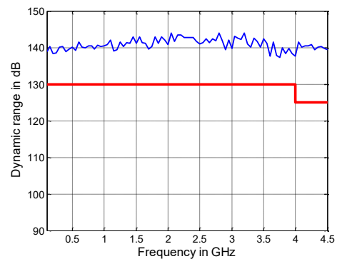
Dynamic range in dB versus frequency of the R&S®ZNB4 1
