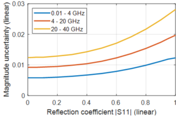
Uncertainty of reflection magnitude and reflection phase measurements of the R&S®ZNB40, model .72 in the frequency range from 10 MHz to 40 GHz; analysis conditions: S_{12} = S_{21} = 0 , cal. power: -10 dBm, meas. power: -10 dBm
