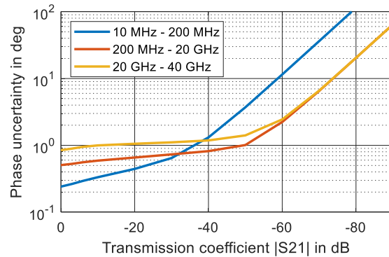
Uncertainty of transmission magnitude and transmission phase measurements of the R&S®ZNB40, model .72 in the frequency range from 10 MHz to 40 GHz; analysis conditions: S_{11} = S_{22} = 0 , cal. power: -10 dBm, meas. power: -10 dBm
