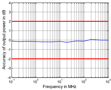
Output power accuracy in dB versus frequency of the R&S ® ZNB20 1
