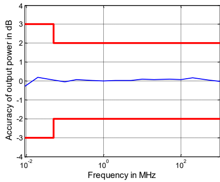
Output power accuracy in dB versus frequency of the R&S ® ZNB8 1
