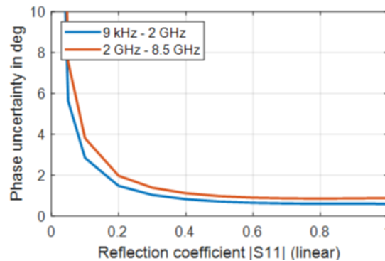
Uncertainty of reflection magnitude and reflection phase measurements of the R&S®ZNB4 1 in the frequency range from 9 kHz to 4.5 GHz, of the R&S®ZNB8 1 in the frequency range from 9 kHz to 8.5 GHz; analysis conditions: S_{12} = S_{21} = 0 , cal. power: -10 dBm, meas. power: -10 dBm
