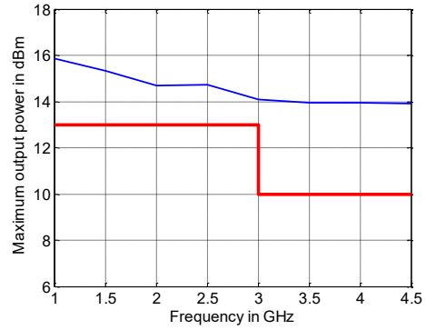
Maximum output power in dBm versus frequency of the R&S ® ZNB4 1
