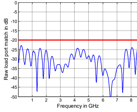
Raw load port match versus frequency of the R&S®ZNB8 1
