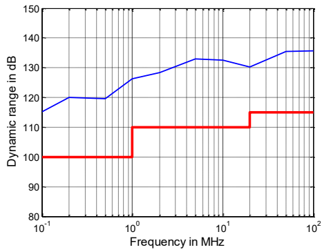
Dynamic range in dB versus frequency of the R&S®ZNB20 1
