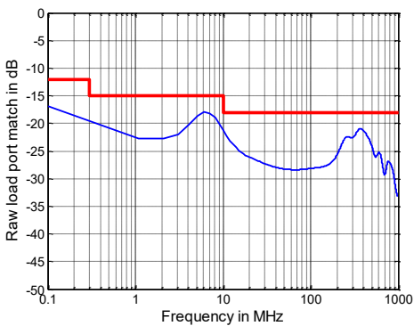
Raw load port match versus frequency of the R&S®ZNB40, models .82 and .84
