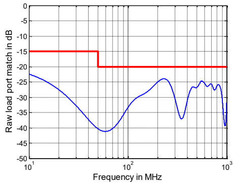
Raw load port match versus frequency of the R&S®ZNB40, model .72
