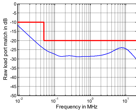
Raw load port match versus frequency of the R&S®ZNB4 1
