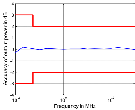
Output power accuracy in dB versus frequency of the R&S ® ZNB4 1
