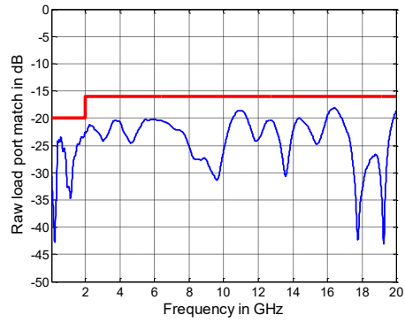
Raw load port match versus frequency of the R&S®ZNB20 1
