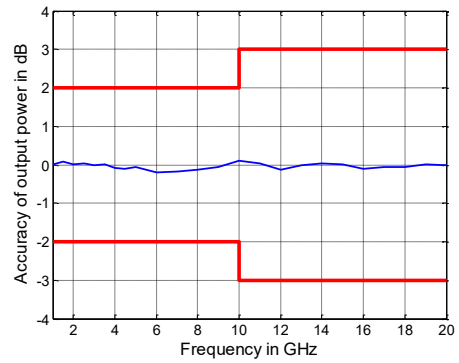
Output power accuracy in dB versus frequency of the R&S ® ZNB20 1
