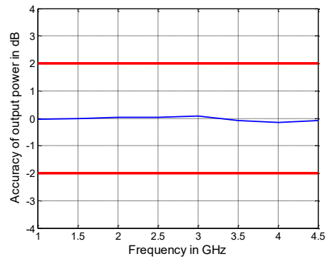
Output power accuracy in dB versus frequency of the R&S ® ZNB4 1
