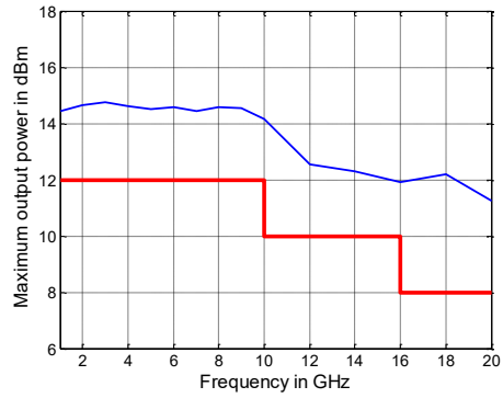
Maximum output power in dBm versus frequency of the R&S ® ZNB20 1
