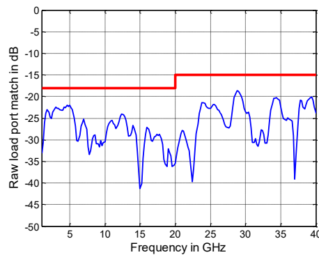
Raw load port match versus frequency of the R&S®ZNB40, models .82 and .84
