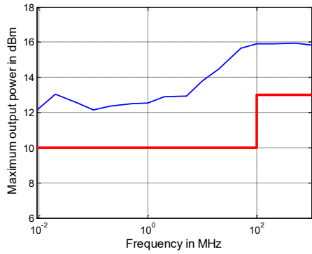
Maximum output power in dBm versus frequency of the R&S ® ZNB4 1
