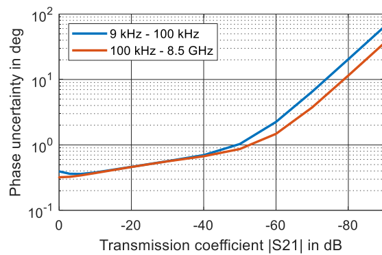
Uncertainty of transmission magnitude and transmission phase measurements of the R&S®ZNB4 1 in the frequency range from 9 kHz to 4.5 GHz, of the R&S®ZNB8 1 in the frequency range from 9 kHz to 8.5 GHz; analysis conditions: S_{11} = S_{22} = 0 , cal. power: -10 dBm, meas. power: -10 dBm
