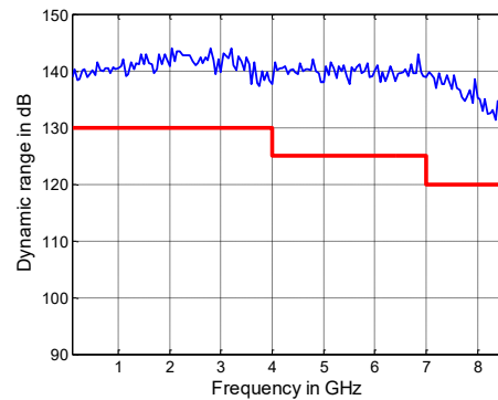
Dynamic range in dB versus frequency of the R&S®ZNB8 1
