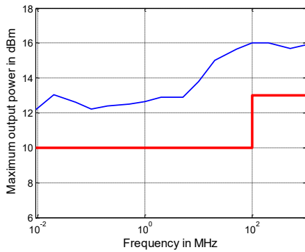
Maximum output power in dBm versus frequency of the R&S ® ZNB8 1
