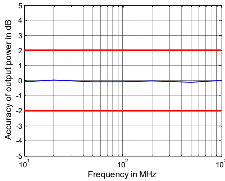
Output power accuracy in dB versus frequency of the R&S ® ZNB40, model .72
