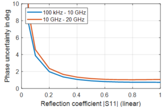
Uncertainty of reflection magnitude and reflection phase measurements of the R&S®ZNB20 1 in the frequency range from 100 kHz to 20 GHz; analysis conditions: S_{12} = S_{21} = 0 , cal. power: -10 dBm, meas. power: -10 dBm
