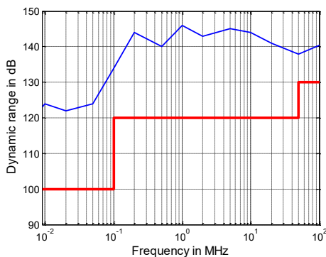
Dynamic range in dB versus frequency of the R&S®ZNB8 1
