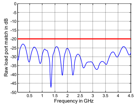
Raw load port match versus frequency of the R&S®ZNB4 1
