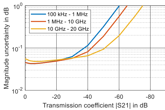
Uncertainty of transmission magnitude and transmission phase measurements of the R&S®ZNB20 1 in the frequency range from 100 kHz to 20 GHz; analysis conditions: S_{11} = S_{22} = 0 , cal. power: -10 dBm, meas. power: -10 dBm
