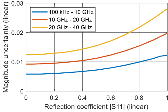
Uncertainty of reflection magnitude and reflection phase measurements of the R&S®ZNB40, models .82 and .84 in the frequency range from 100 kHz to 40 GHz; analysis conditions: S_{12} = S_{21} = 0 , cal. power: -10 dBm, meas. power: -10 dBm
