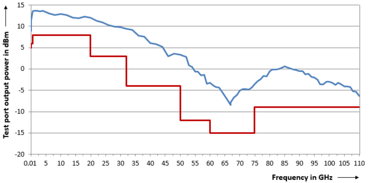
Test port output power in dBm versus frequency of the R&S®ZVA110 (models .13 and .15)
