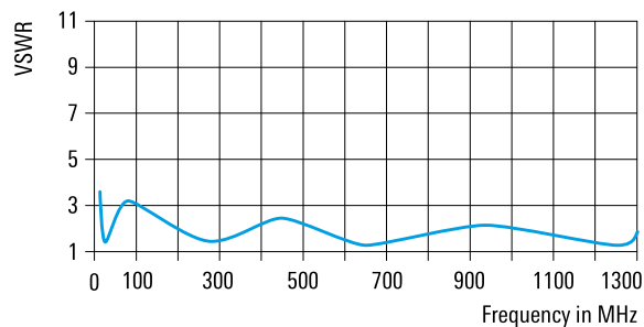
Typical VSWR
