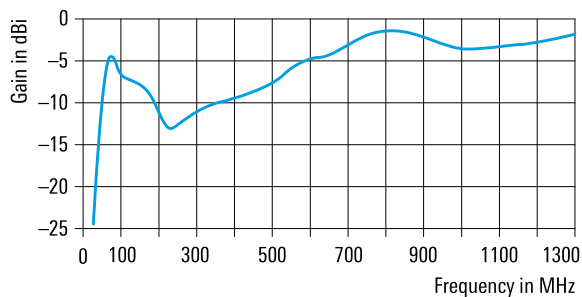
Typical gain
