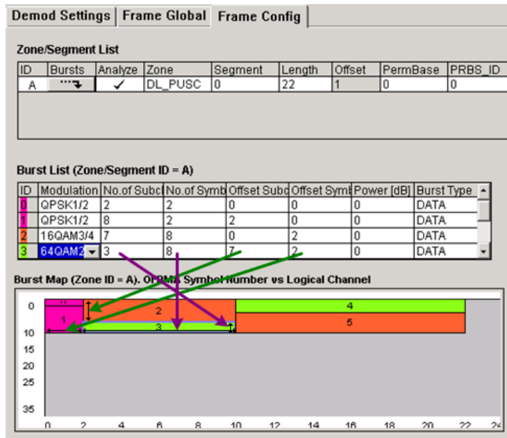
Figure 4-15: Definition of the Burst Offset [green arrows] and the Burst Length [violet arrows] parameters from the Burst List
