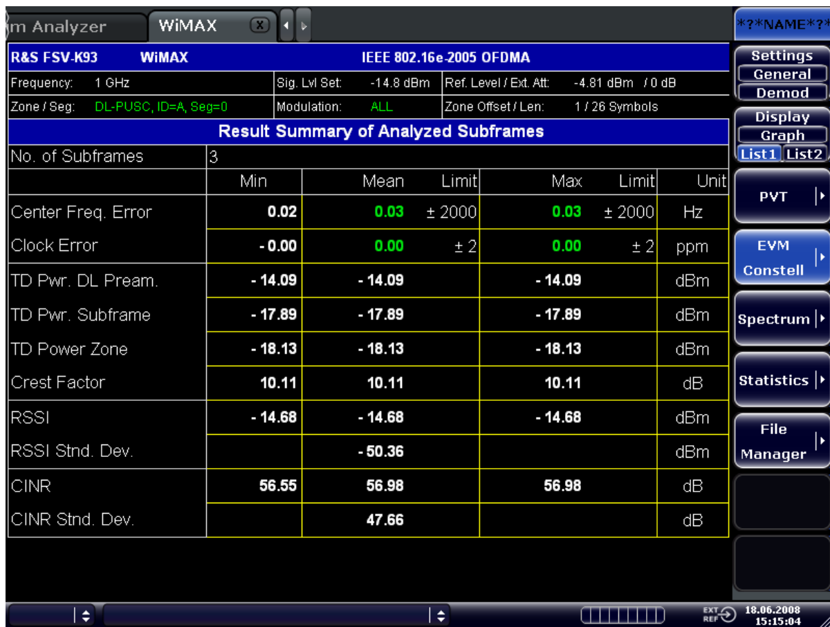
Figure 4-4: Result summary list for IEEE 802.16e-2005 OFDMA/WiBro (example)
