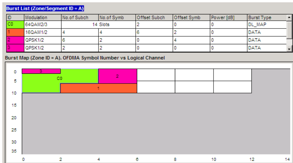
Figure 4-16: Zone containing a wrapping DL_MAP burst (C0).
