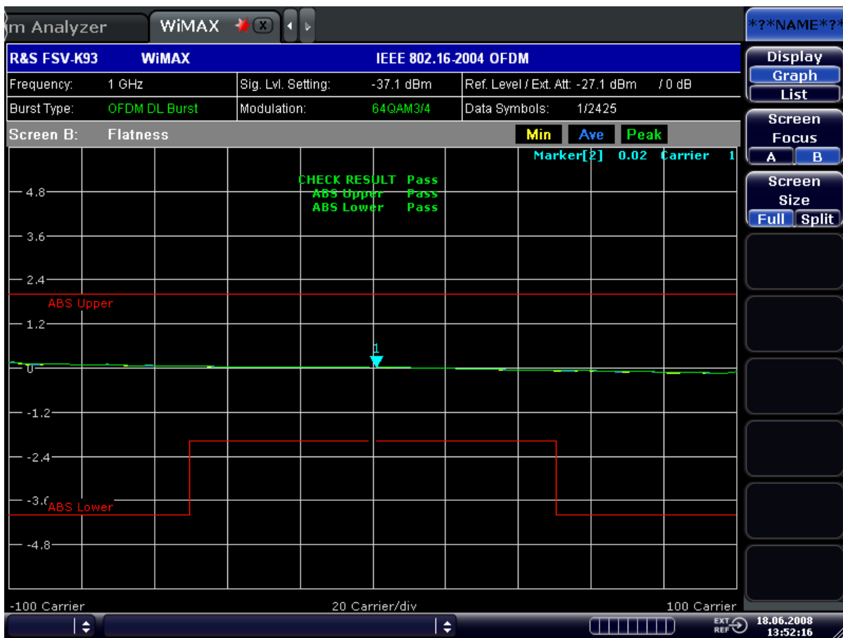
Figure 3-2: Spectrum Flatness
