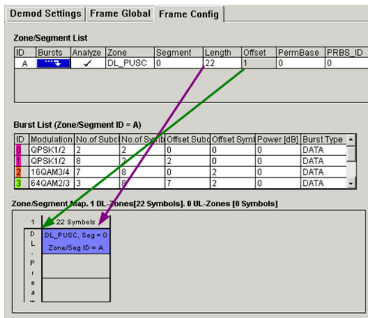
Figure 4-14: Definition of the Zone Offset [green arrow] and the Zone Length [violet arrow] parameters from the Zone/Segment List
