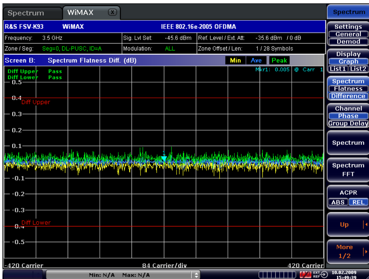
Figure 4-11: Spectrum Flatness Difference for IEEE 802.16e-2005 OFDMA
