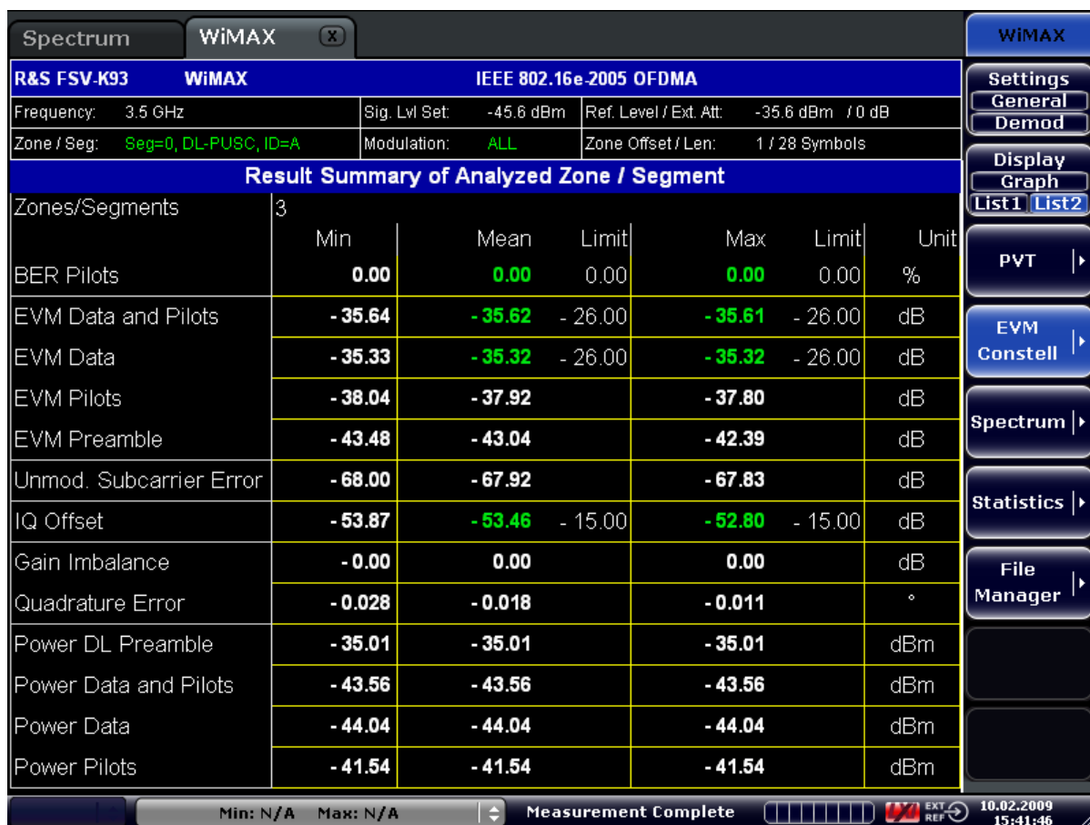
Figure 4-5: Result summary list 2 for IEEE 802.16e-2005 OFDMA/WiBro (example)
