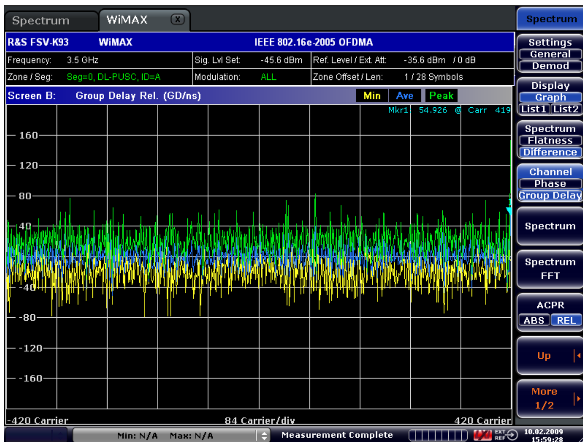
Figure 4-13: Group Delay for IEEE 802.16e-2005 OFDMA/WiBro
