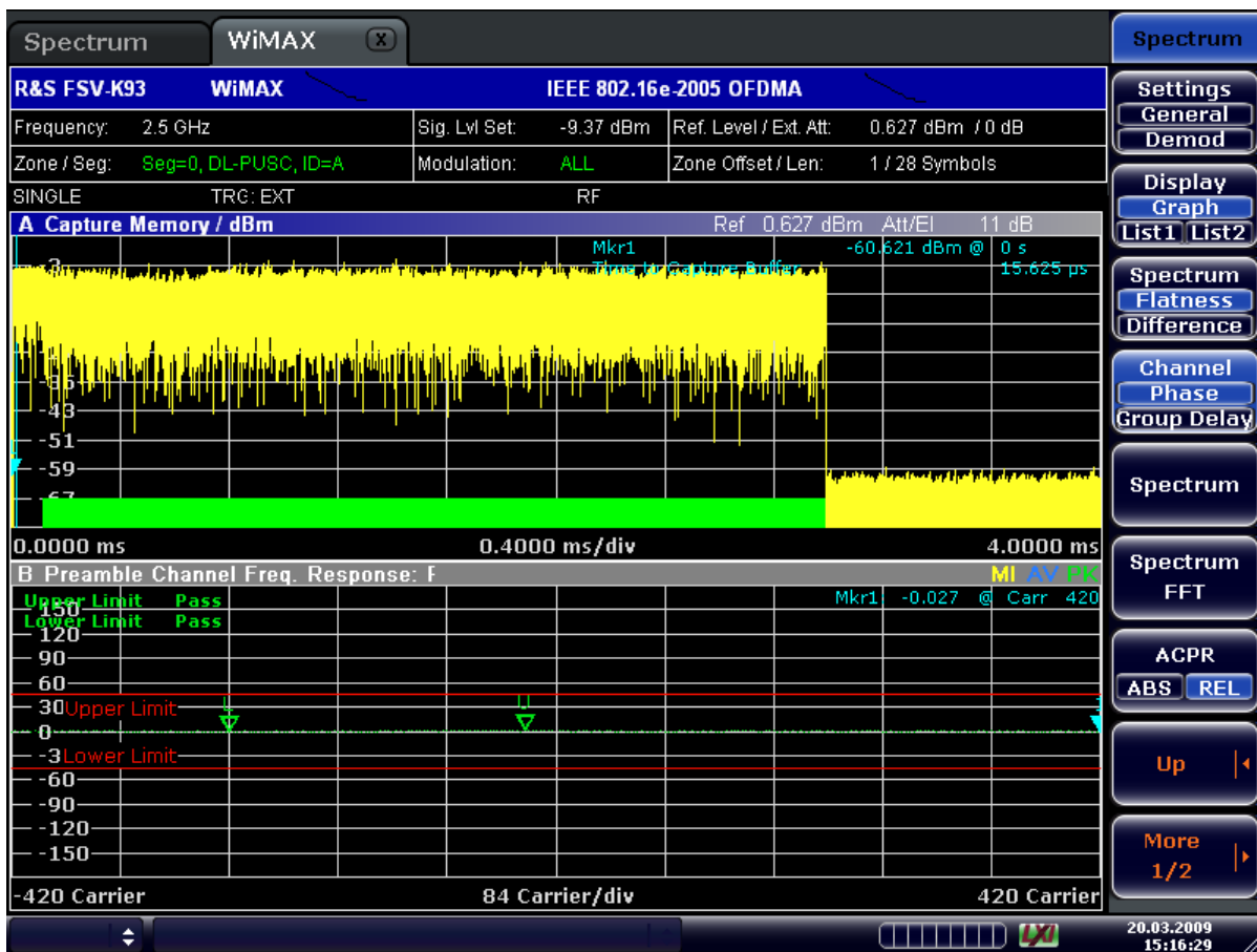
Figure 4-12: Preamble Channel Frequency Response Phase for IEEE 802.16e-2005 OFDMA
