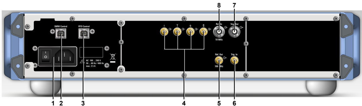
Figure 4-2: Rear view of the R&S UD1065
