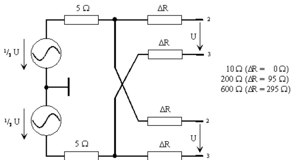
Bild 5-7: Channel = 2 = 1
