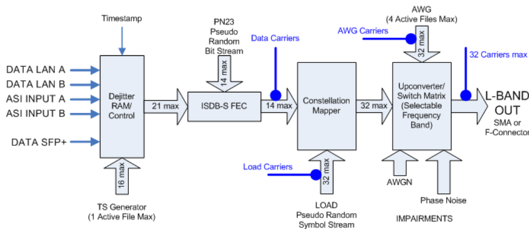
Block Diagram for ISDB-S 32 Mode
