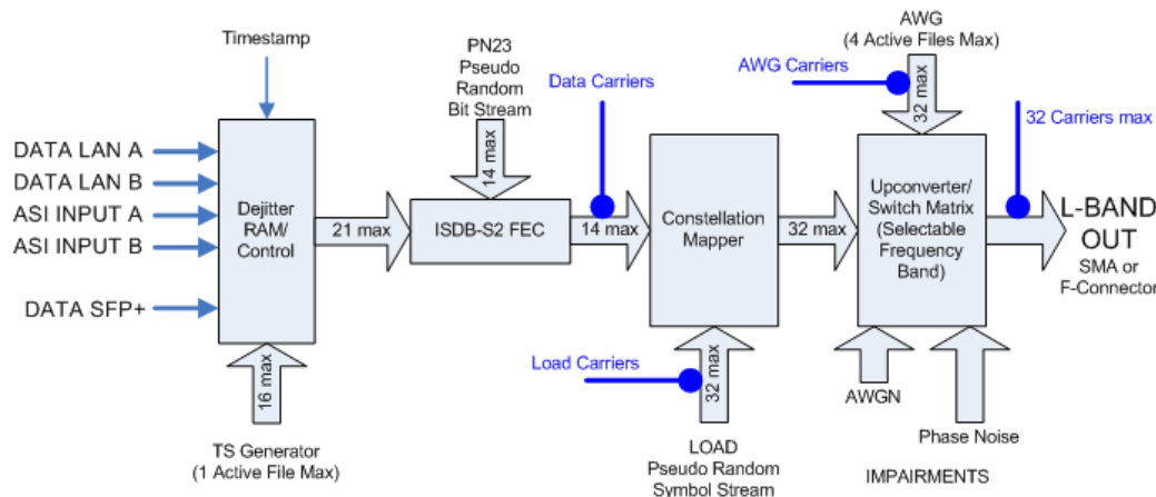
Block Diagram for ISDB-S2 32 Mode
