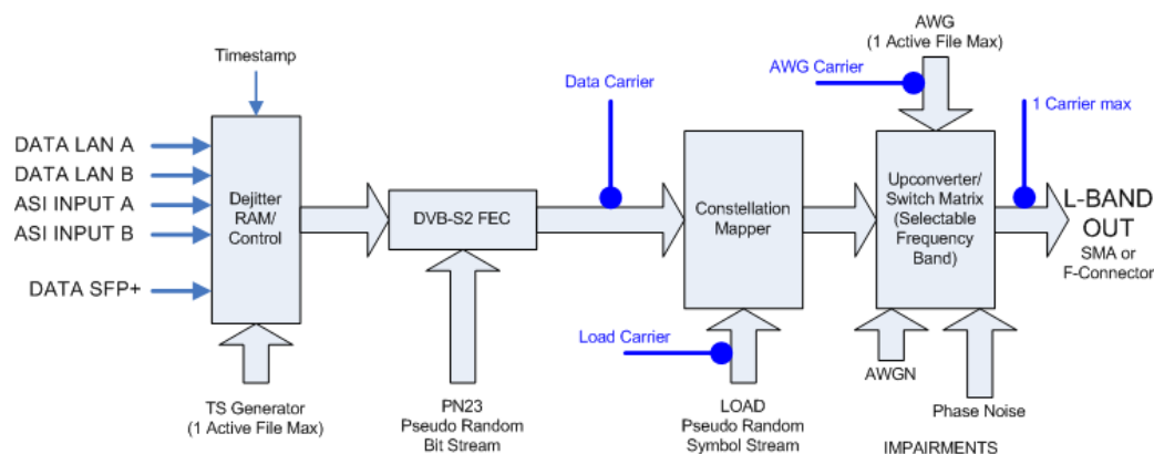
Block Diagram for DVB 1 Mode
