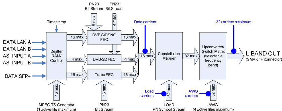
Block Diagram for Turbo 32 Mode
