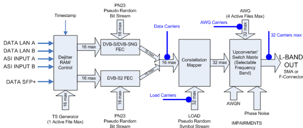
Block Diagram for DVB 32 Mode
