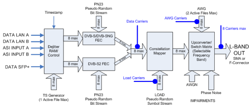
Block Diagram for DVB 8 Mode
