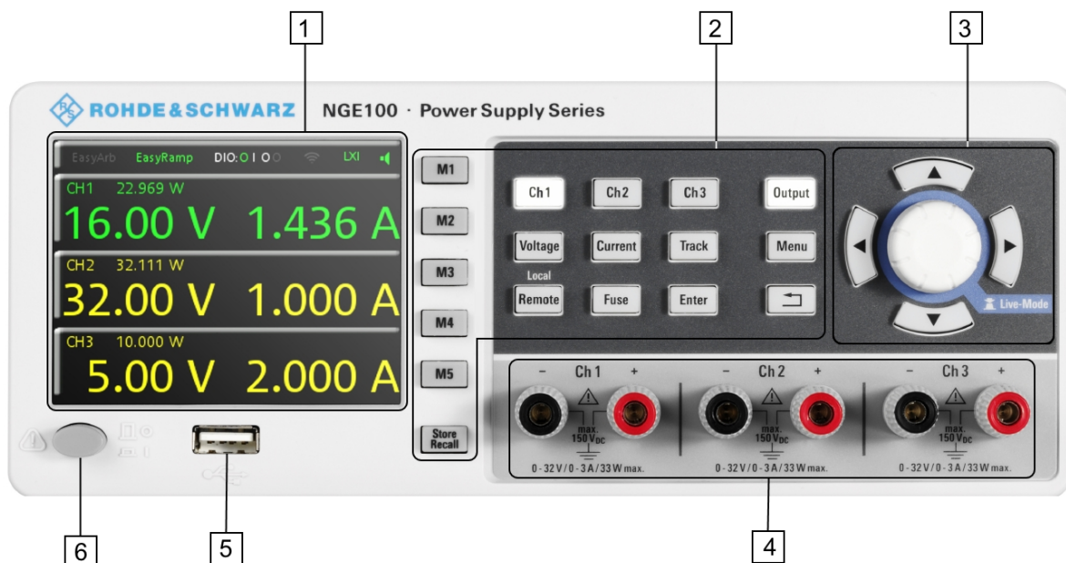
Figure 4-1: Front panel of R&S NGE100
