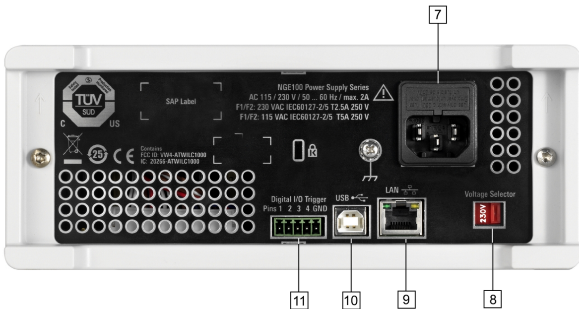
Figure 4-2: Rear panel of R&S NGE100
