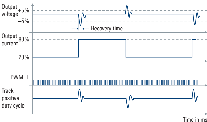
Figure 2: Load transient response
