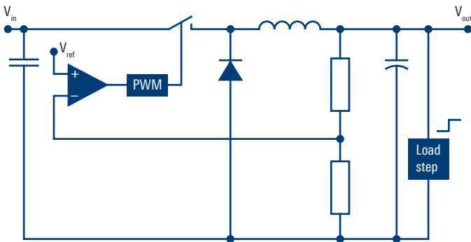
Figure 1: Load transient setup of a step-down converter
