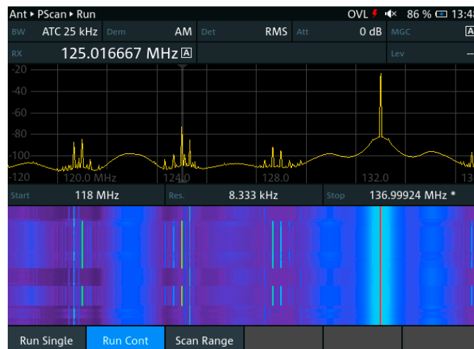
Intuitive spectrum monitoring with the R&S®PR200.
