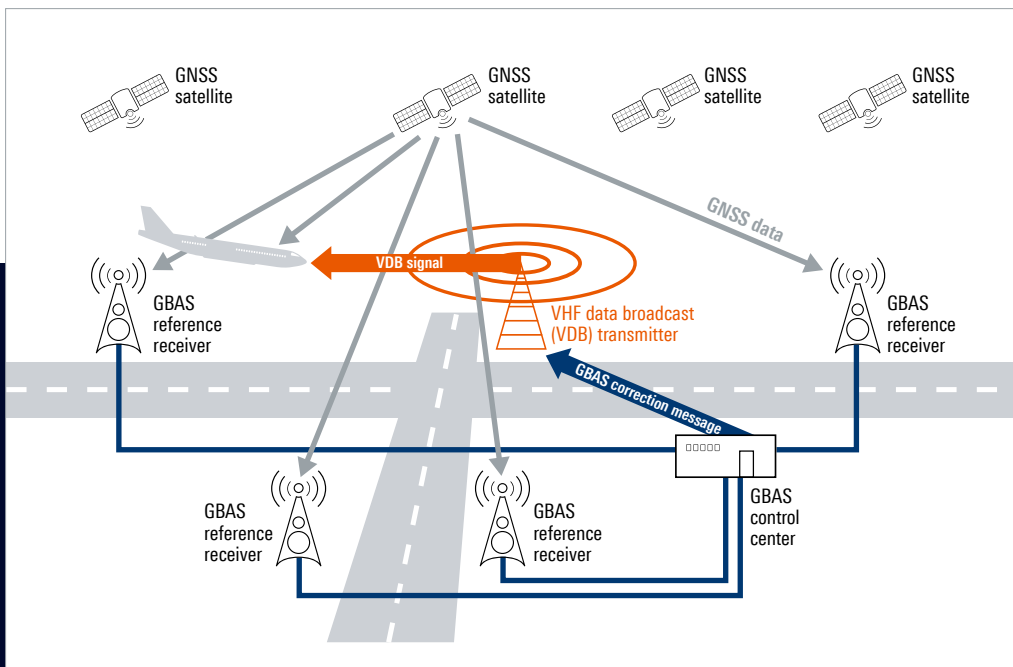
GBAS components and signals (simplified representation).
