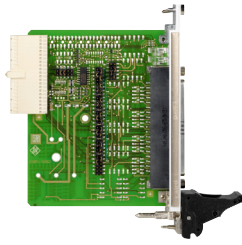
R&S®TS-PRIO4, rear I/O transmission module for R&S®TS-PIO3B and R&S®TS-PMB
