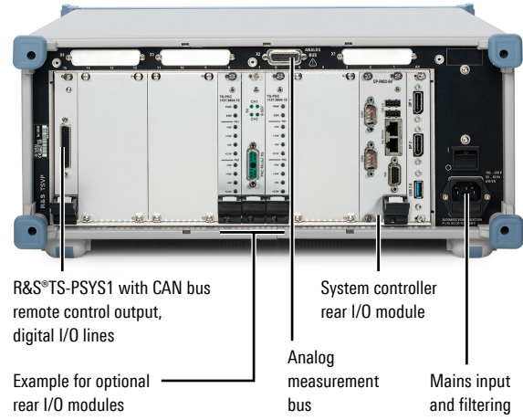
R&S®CompactTSVP rear view
