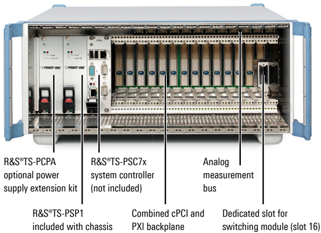
R&S®CompactTSVP front view
