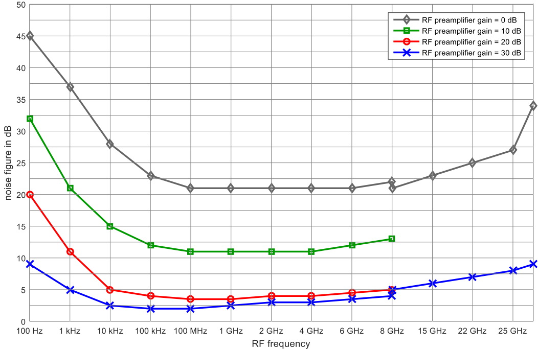
Typical noise figure with R&S®FSWT-B23 or R&S®FSWT-B223 option, RF preamplifier on
