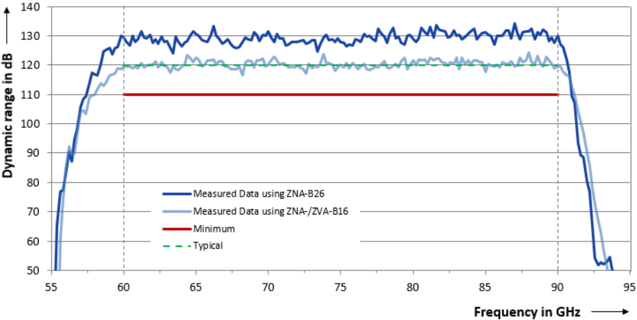
Dynamic range versus frequency of the R&S ® ZC90
