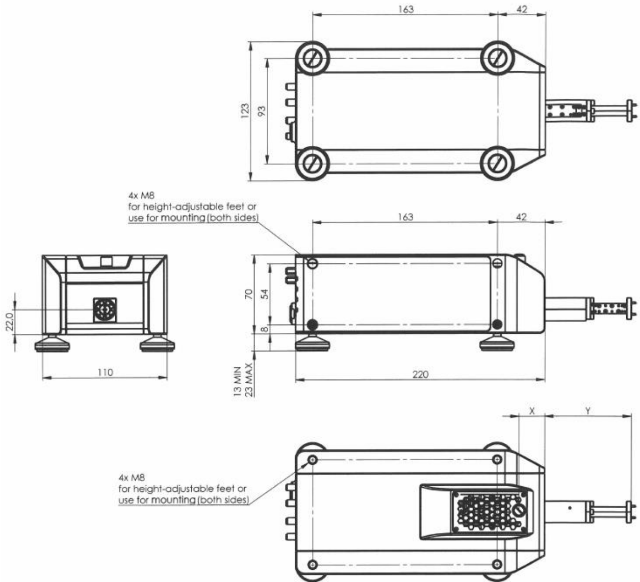
Dimensions (in mm) of the R&S®ZC90 and R&S®ZC110 millimeterwave converters
