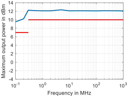
Typical maximum output power in dBm versus frequency of the R&S®ZNB43
