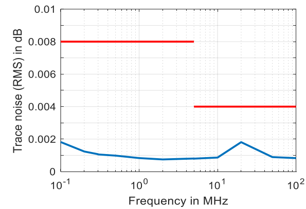
Typical trace noise (RMS) in dB versus frequency of the R&S®ZNB26
