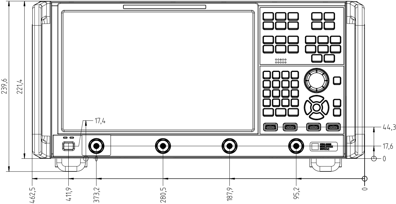
Front view of the R&S®ZNB
