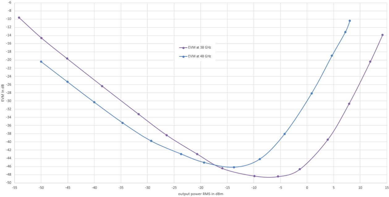
EVM values versus output power at different center frequencies in combination with an R&S®SMW200A (IF mode: low)
