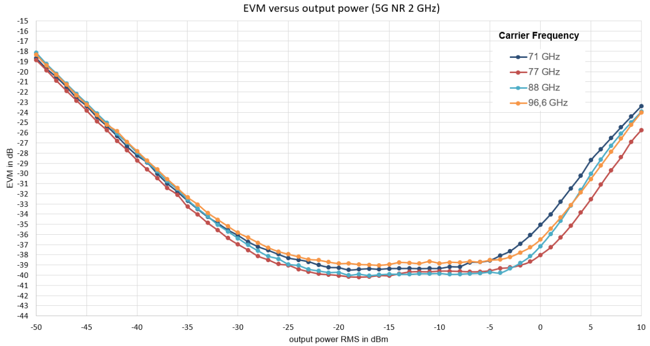
EVM values versus output power at different center frequencies with R&S®SMW200A (with R&S®SMW-B711 option) in combination with R&S®FE110SR and R&S®FSW (with R&S®FSW-B4001 option), IF mode: EVM optimized
