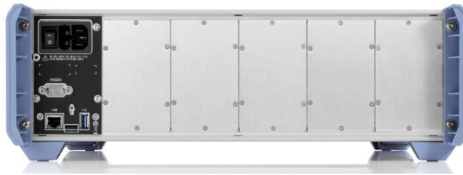
Rear view R&S®OSP320, rear module slots RS01 to RS05 (from left to right without options)
