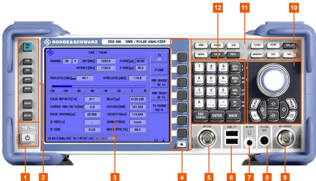
Figure 5-1: Front panel view of the R&S EDS300
