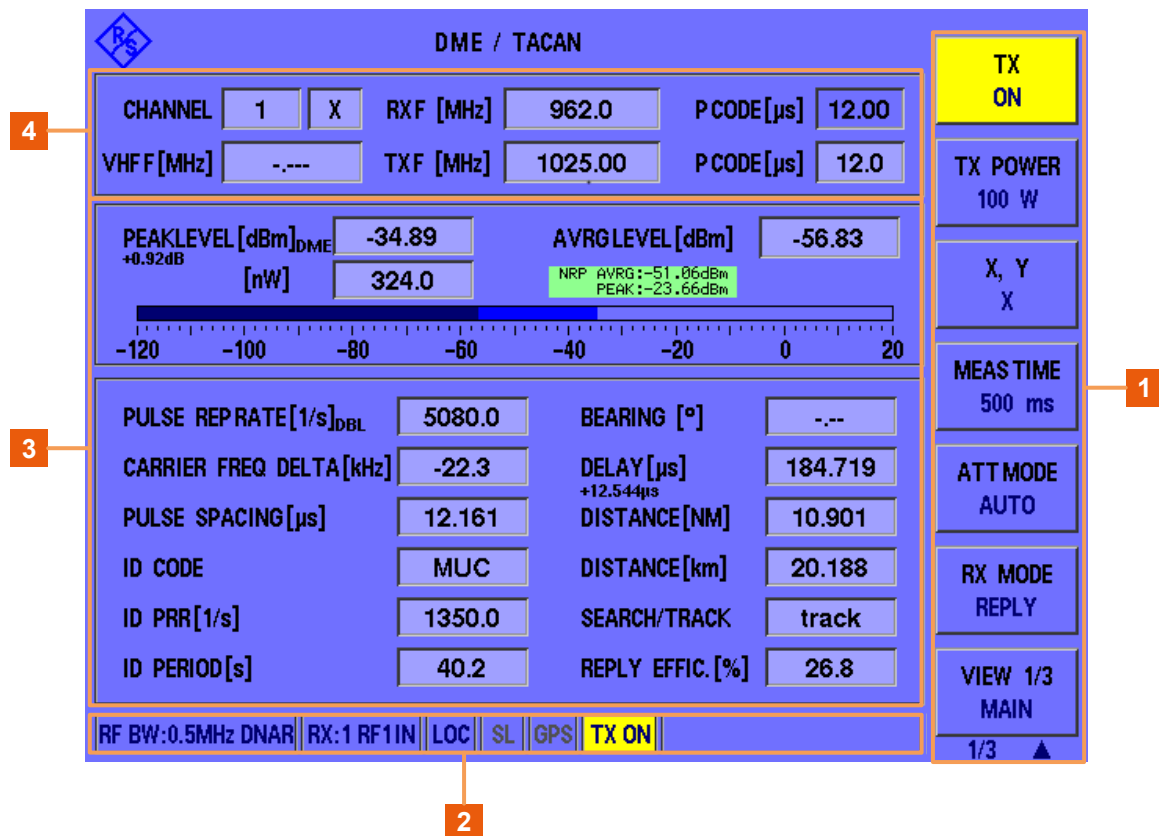
Figure 6-1: Typical R&S EDS300 screen display (using DME mode as an example)
