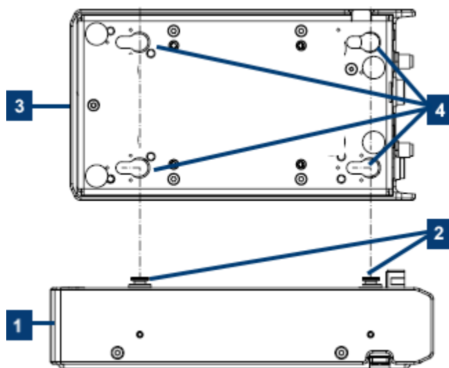
Figure 5-1: Example: Aligning R&S TSMA6/6B-BP and R&S TSME6
