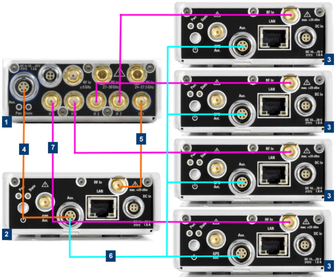
Figure 6-1: Example measurement setup with 5 R&S TSME6 scanners
