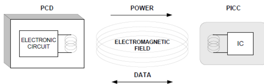
Figure 4-1: PCD (contactless reader) and PICC (transponder) configuration
