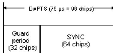
Figure 2-2: Structure of DwPTS
