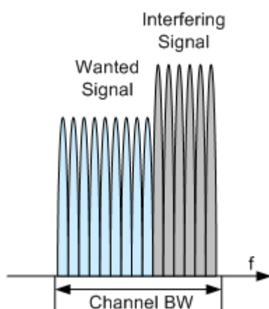
Figure 7-6: Example: In-channel selectivity (ICS), Channel BW = 3 MHz, Frequency Allocation = Lower Frequency
