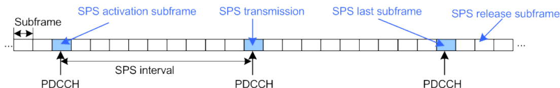
Figure 2-21: Semi-persistent scheduling (SPS)
