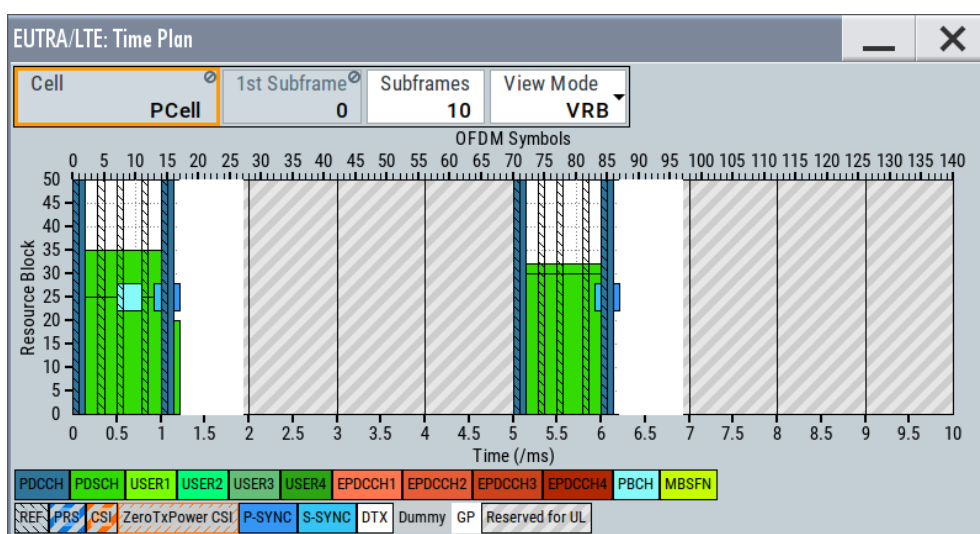
Figure 6-1: TDD time plan (DL)
