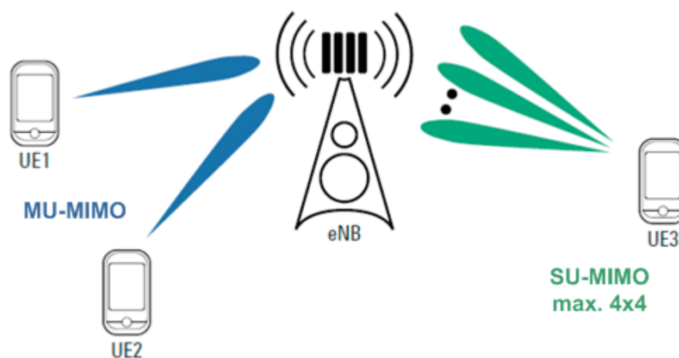
Figure 2-30: Supported transmit layers in LTE-Advanced (uplink)
