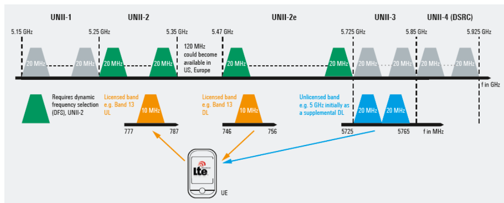
Figure 2-33: Carrier aggregation of licensed and unlicensed spectra [Rohde & Schwarz poster "Evolution of Carrier Aggregation (3GPP Releases 10 to 13)"]
