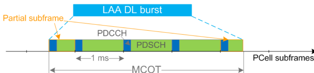
Figure 2-34: DL LAA burst transmission
