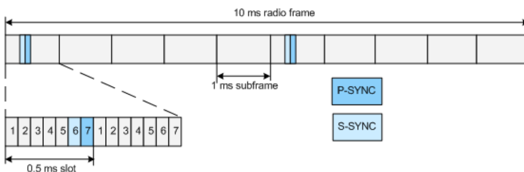
Figure 2-10: P-SYNC and S-SYNC structure (normal CP; 1.25 MHz bandwidth)
