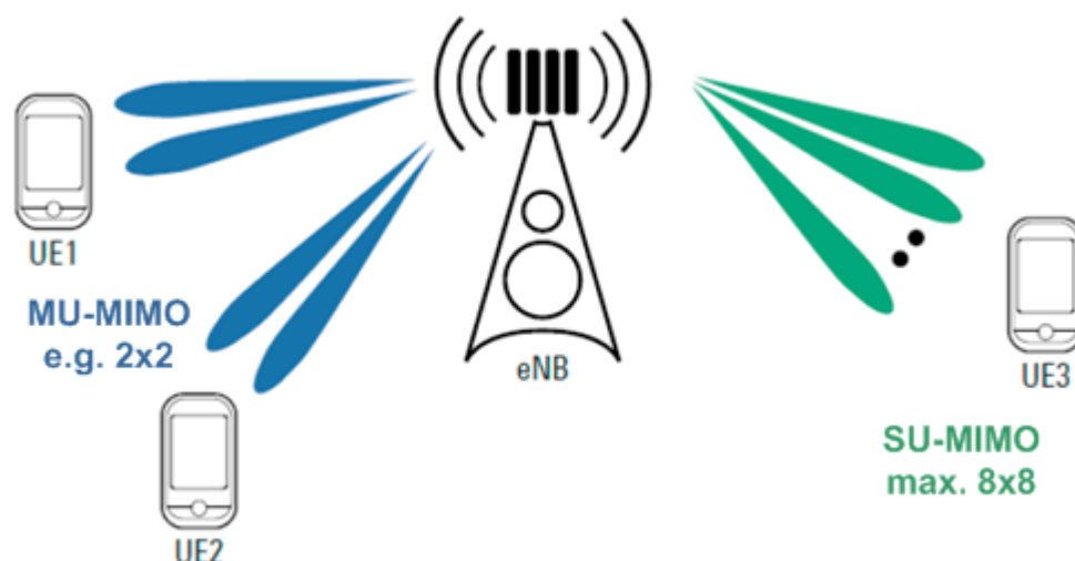
Figure 2-29: Supported transmit layers in LTE-Advanced (downlink)
