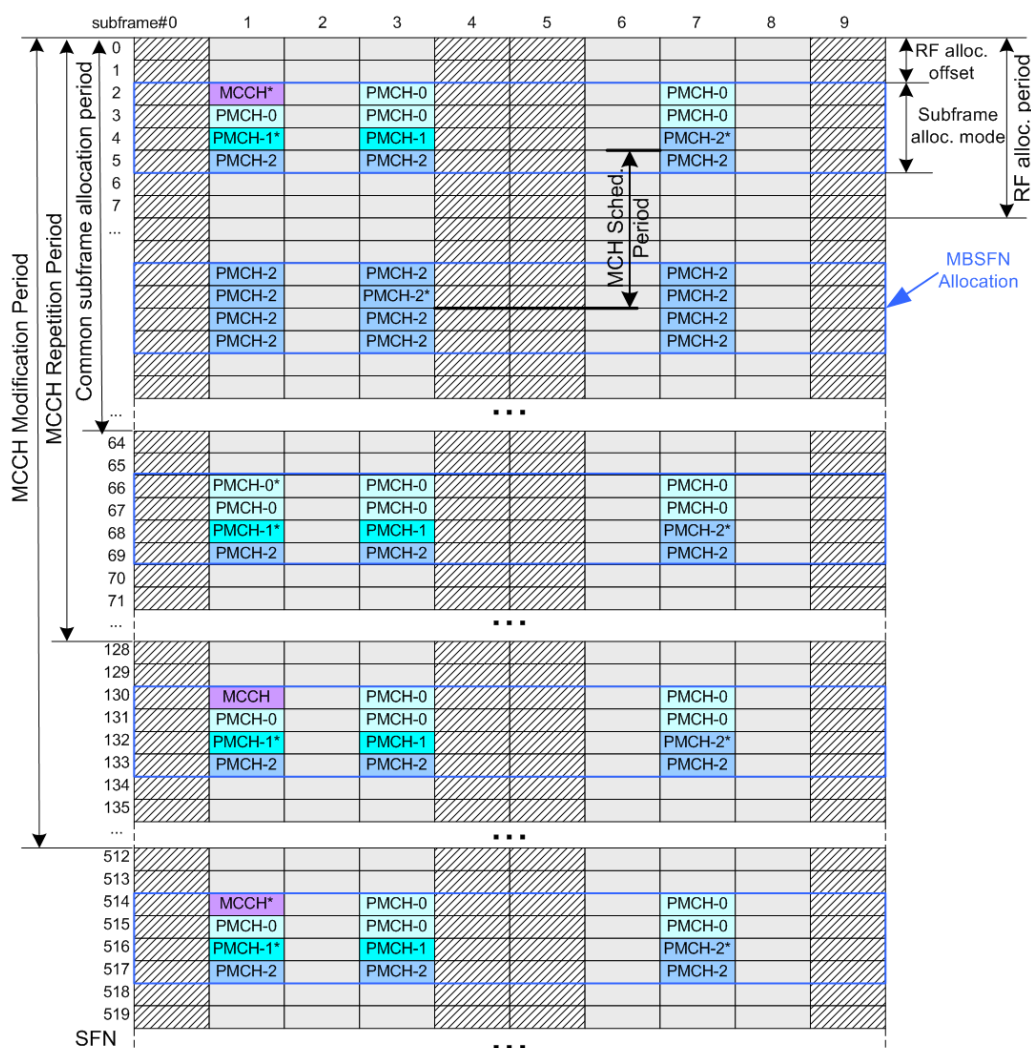
Figure 4-4: Example of MBSFN resource allocation
