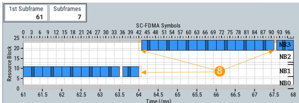
Figure 5-8: Narrowband hop with PUSCH-to-PUSCH transition
