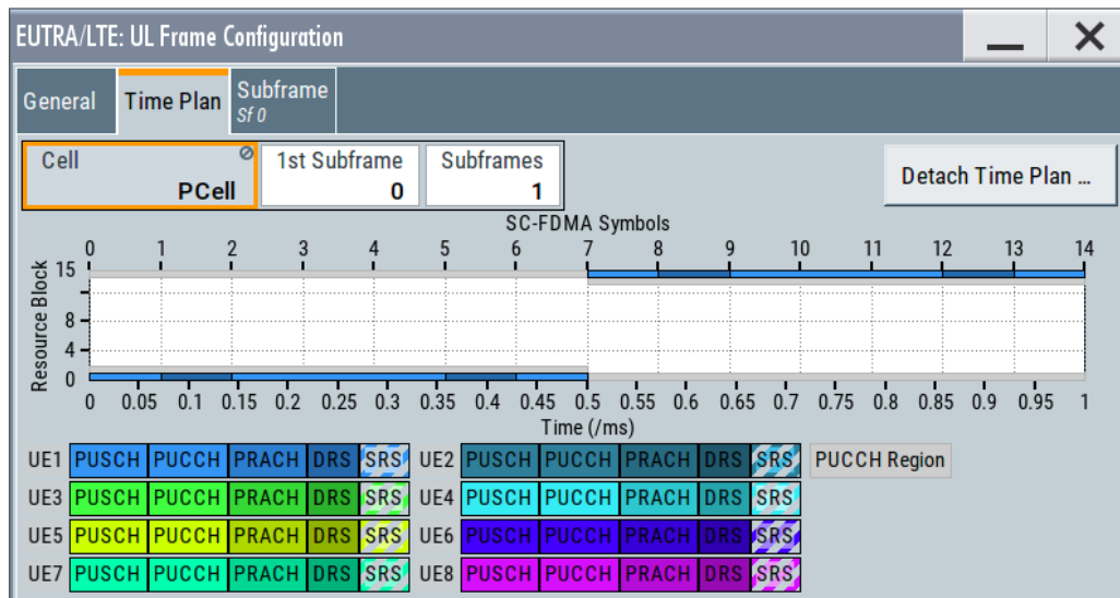
Figure 5-21: Example: Representation of subframe with PUCCH region with three reserved resource blocks on the time plan
