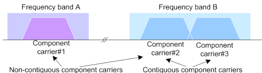
Figure 2-26: Carrier aggregation
