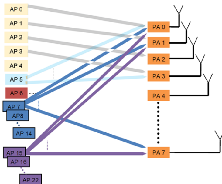
Figure 2-8: Mapping of logical antenna ports to physical transmit antennas (3GPP Rel. 10)
