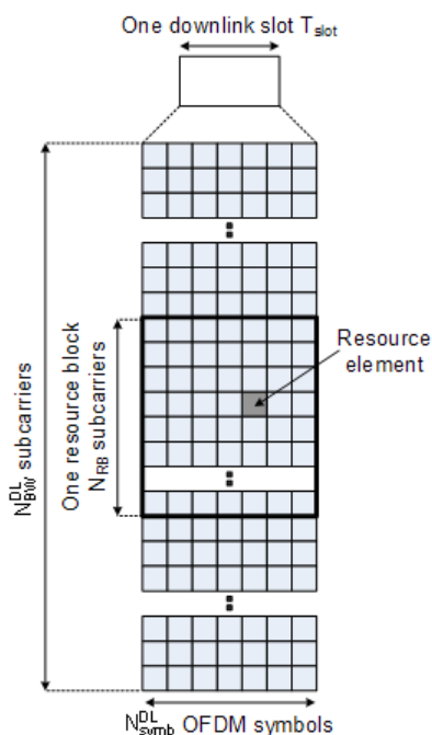
Figure 2-6: Downlink resource grid (3GPP TS 36.211)
