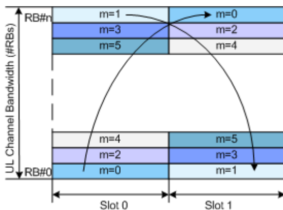
Figure 2-18: PUCCH mapping
