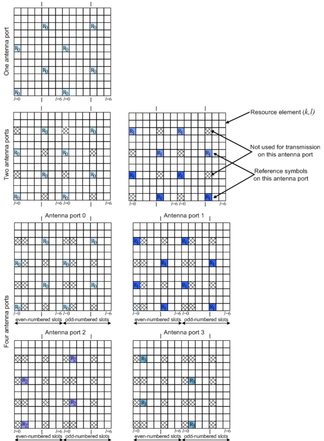
Figure 2-9: Downlink reference signal structure (normal cyclic prefix)
