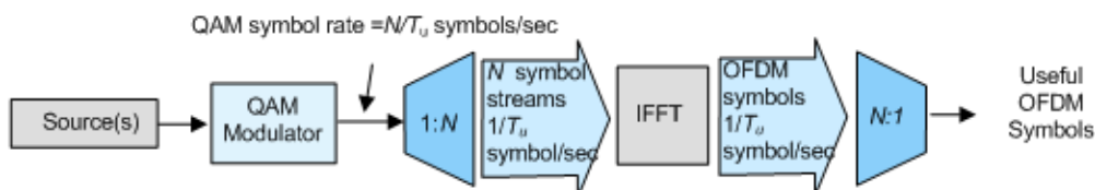
Figure 2-2: OFDM signal generation chain (3GPP TR 25.892)
