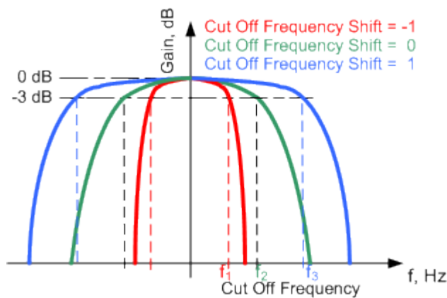
Figure 9-2: Example of the frequency response of a filter with different cutoff frequency shift
