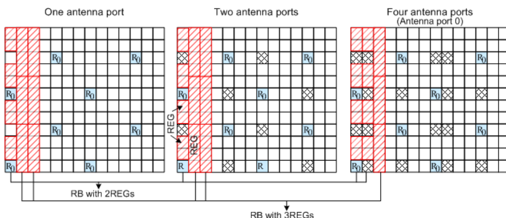
Figure 2-7: Resource elements groups (REG)
