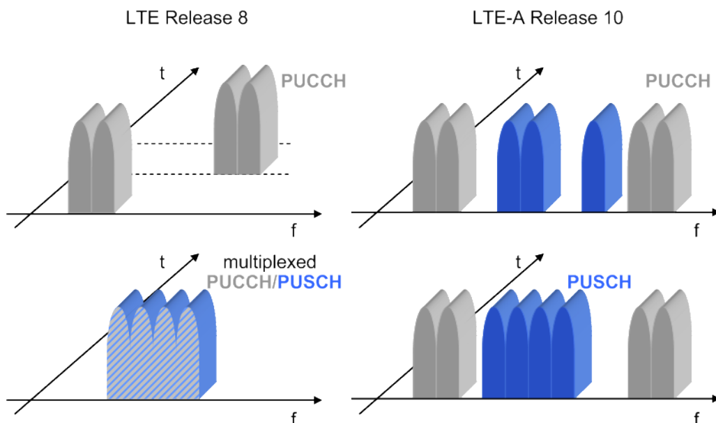
Figure 2-28: LTE Release 8 and LTE-A Release 10 UL transmission schemes
