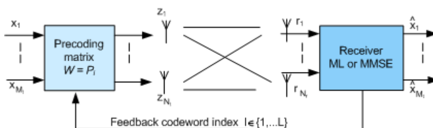
Figure 2-24: Precoding principle
