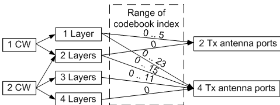
Figure 2-31: Codeword to layer mapping for uplink spatial multiplexing (LTE Rel. 10)
