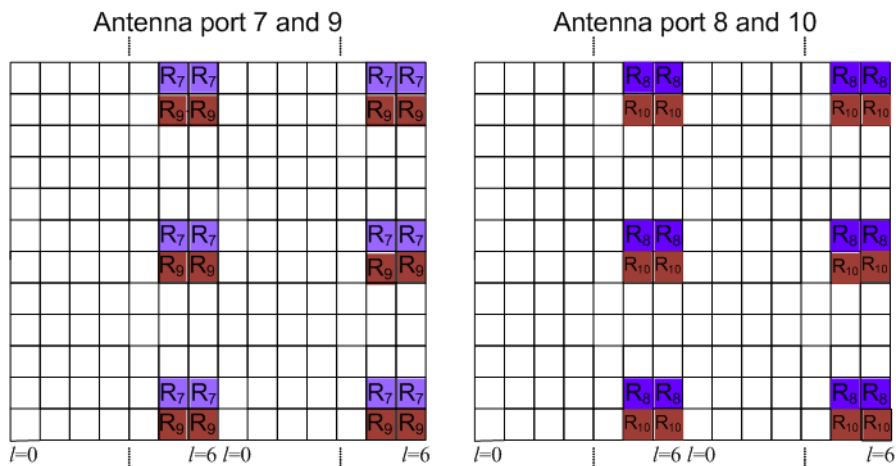
Figure 2-13: UE-specific reference signals, antenna ports 7 to 10 (normal cyclic prefix, downlink sub-frame)
