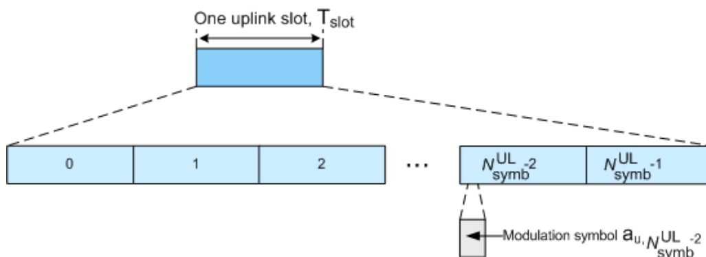
Figure 2-17: Uplink slot structure
