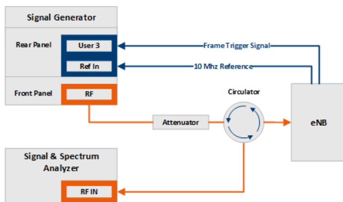
Figure 7-3: Test setup for Test case 6.7: Transmitter Intermodulation
