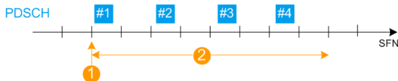
Figure 5-2: PDSCH carrying SIB1-BR transmission (Channel Bandwidth = 10 MHz)
