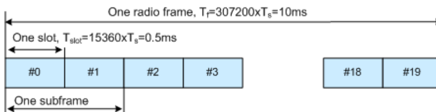
Figure 2-3: Frame format 1 (FDD mode)
