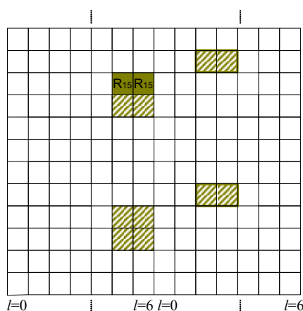
Figure 2-15: Mapping of a CSI-RS on antenna port 15 (CSI configuration 0, normal cyclic prefix)
