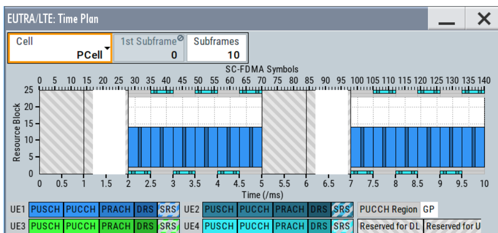
Figure 6-2: TDD time plan (UL)
