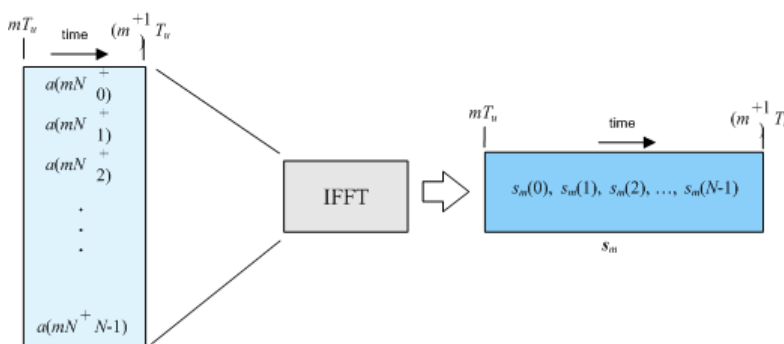
Figure 2-1: OFDM useful symbol generation using an IFFT (3GPP TR 25.892)
