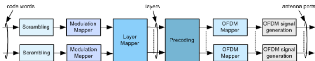
Figure 2-25: Overview of downlink baseband signal generation
