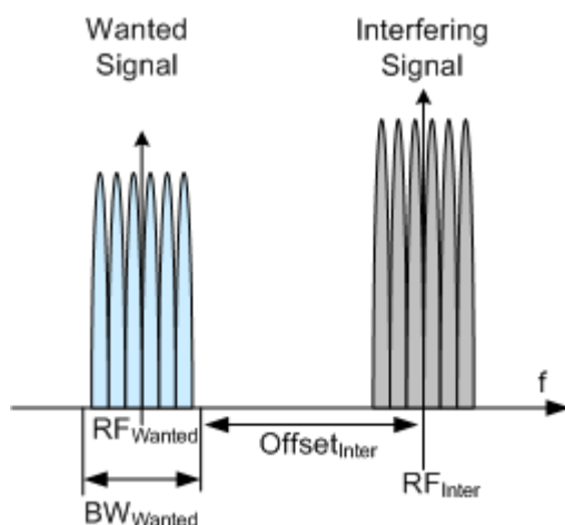
Figure 7-5: Example: Adjacent Channel Selectivity (ACS), Channel BW = 1.4 MHz
