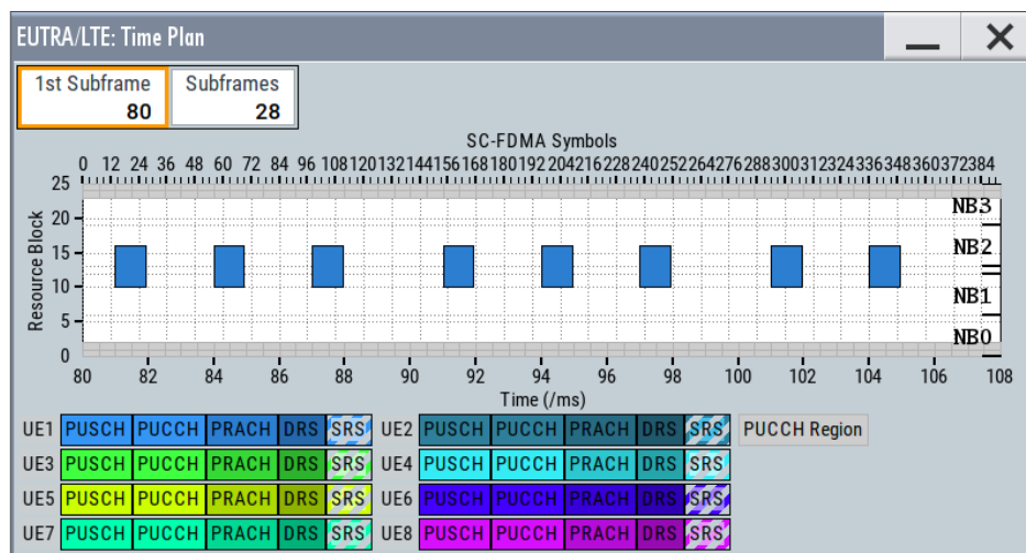
Figure 5-22: PRACH configuration visualization in the "Time Plan" ("PRACH Configuration = 9", "Repetitions = 8"; PRACH bandwidth = 6 RB)
