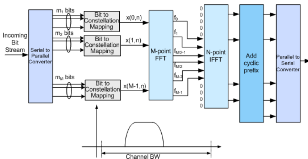
Figure 2-16: Block diagram of DFT-s-OFDM (localized transmission)
