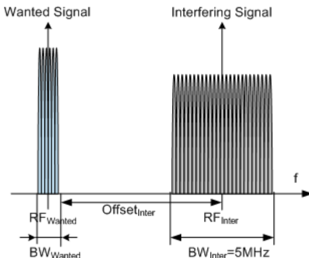
Figure 7-4: Example: Offset to Channel Edge (Channel Bandwidth = 1.4 MHz)
