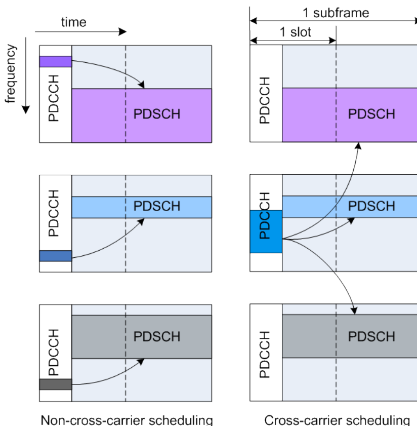
Figure 2-27: LTE-A scheduling approaches
