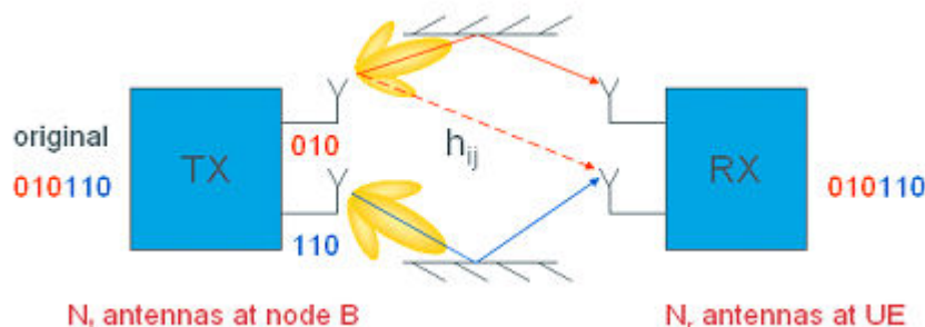
Figure 2-22: Spatial multiplexing
