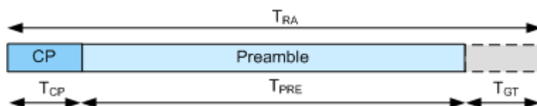
Figure 2-20: Random access preamble
