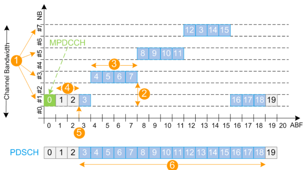
Figure 5-3: Example of PDSCH hopping
