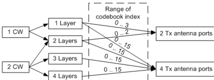
Figure 2-23: Codeword to layer mapping for downlink spatial multiplexing (LTE Rel. 8/9)
