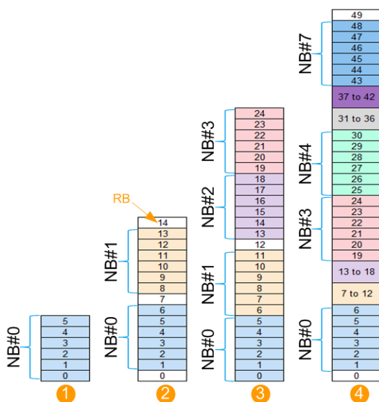
Figure 5-1: eMTC narrowbands
