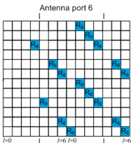
Figure 2-14: Mapping of PRS (normal cyclic prefix), one and two PBCH antenna ports.
