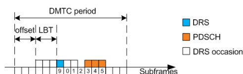
Figure 2-35: DRS allocation
