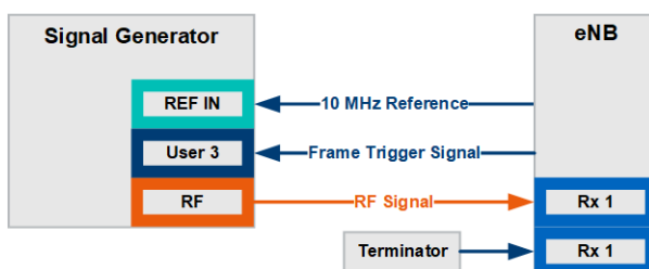
Figure 7-1: One Path Standard Test Setup (Example of simulating the test case 7.3 "Dynamic Range")
