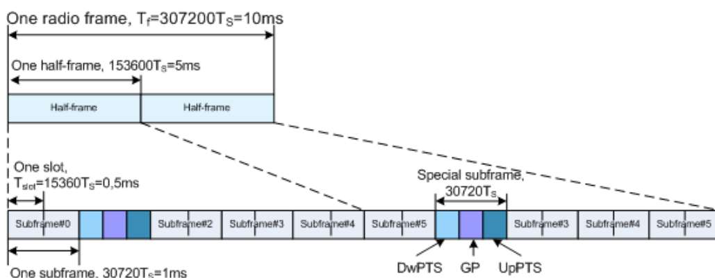
Figure 2-4: Frame format 2 (TDD mode), 5 ms switching periodicity
