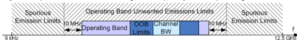
Figure 7-2: Transmitter tests frequency limits
