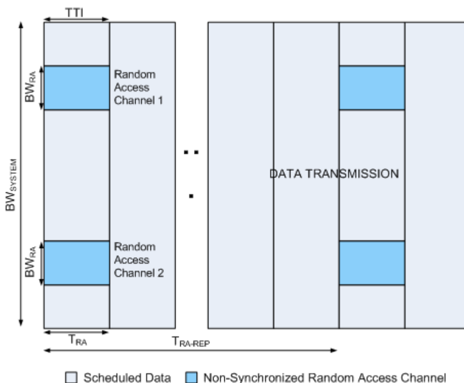
Figure 2-19: Random access structure, principle
