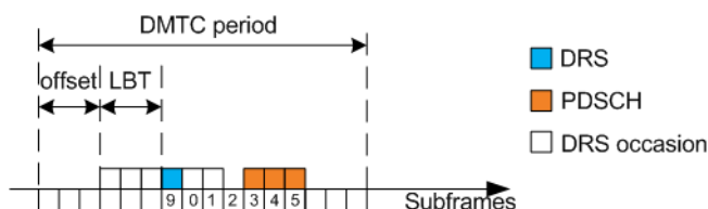
Figure 4-5: DRS allocation
