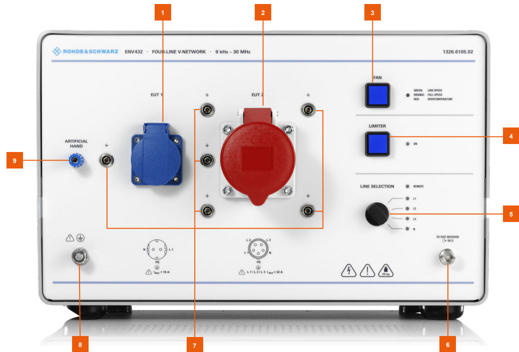
Figure 2-1: Front view
